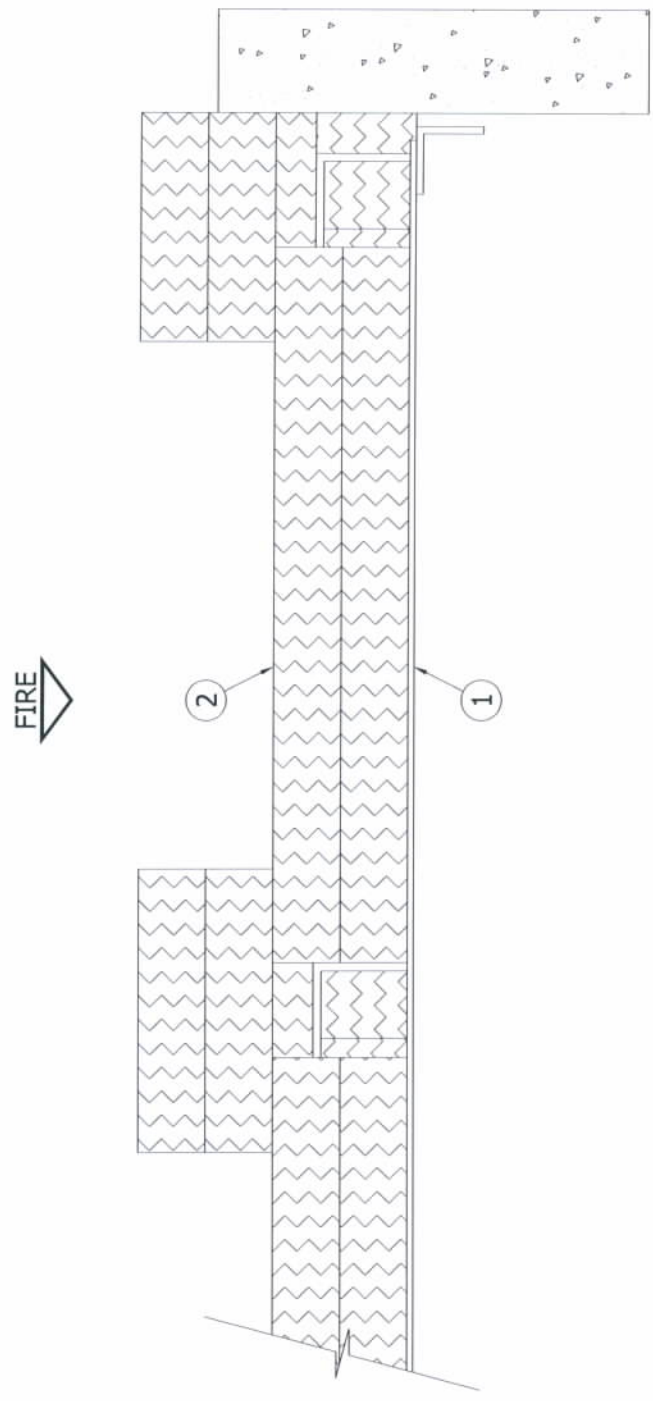
Figure 2 – Detail A
